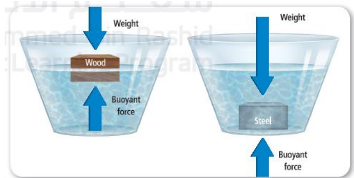
Figure 13 The steel block sinks because the buoyant force from the fluid is less than the gravitational force on the object. When the buoyant force is the same as or greater than the gravitational force—as with the wooden block—the object floats.
