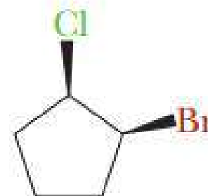
1 -Bromo-2-chlorocyclopentane
