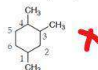
-not- 1,3,4-Trimethylcyclohexane (1 + 3 + 4 = 8)
