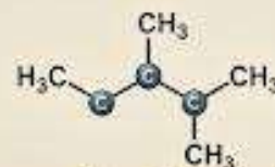
branched chains
