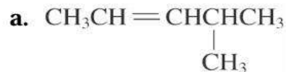
4-methyl-2-pentene
