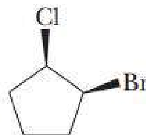
Cyclopentane
