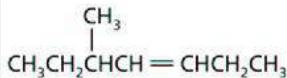
5-methyl-3-heptene
