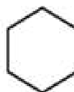
Line structure
