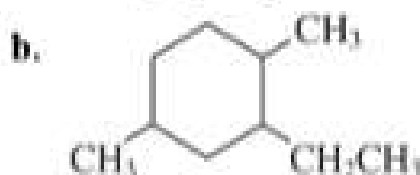
2-ethyl-1,4-dimethylcyclohexane
