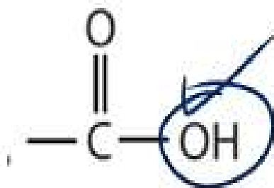
carboxyl
