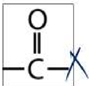
carbonyl
