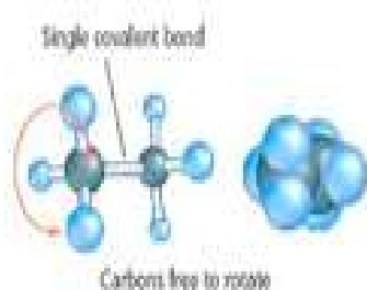
Ethane
