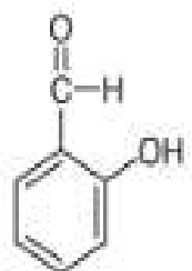
salicylaldehyde
