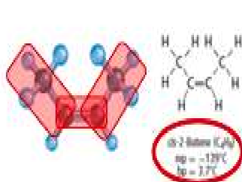
cis-
