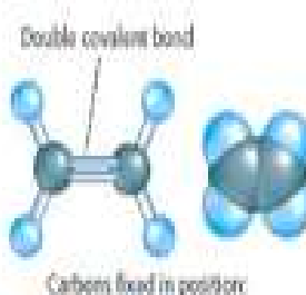
Ethene
