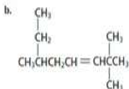
2,2,6-trimethyl-3-octene
