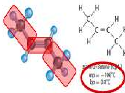
trans-
