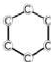
Skeletal structure
