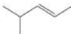
compound D
