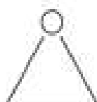
compound B
