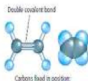
Ethene
