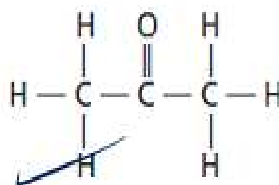
2-Propanone (acetone)
