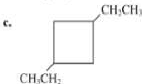
1,3-diethylcyclobutane
