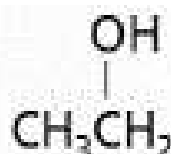
Ethanol
