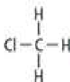
Chloromethane
