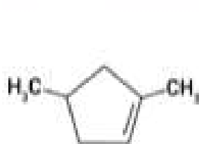
compound A
