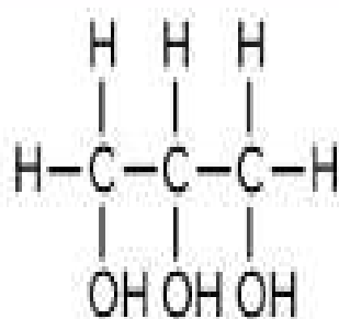
1,2,3-Propanetriol (glycerol)
