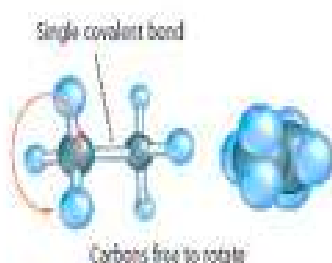
Ethane
