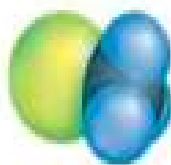
Chloromethane
